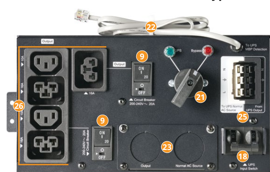
Model MBP6KIECG2 maintenance bypass module (0U)
